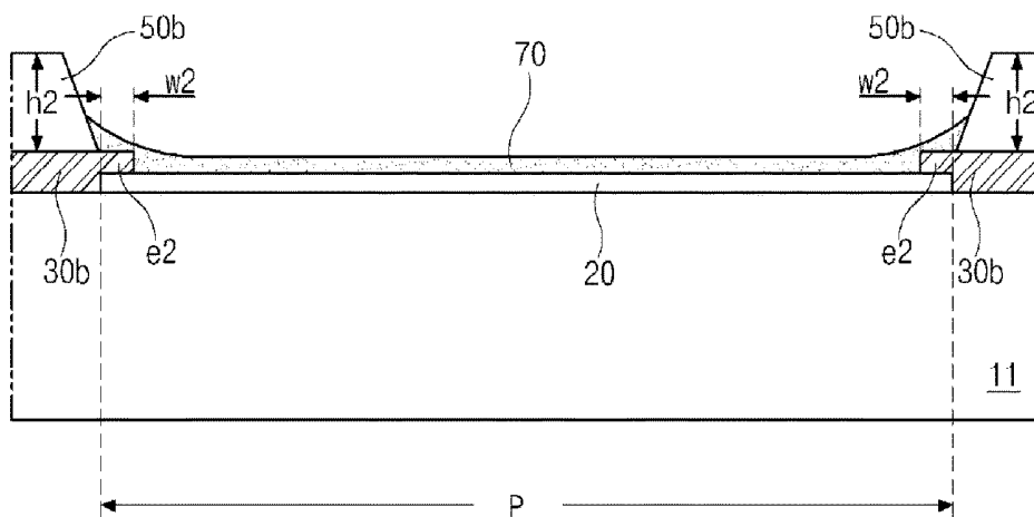
FIG. 3 RELATED ART
