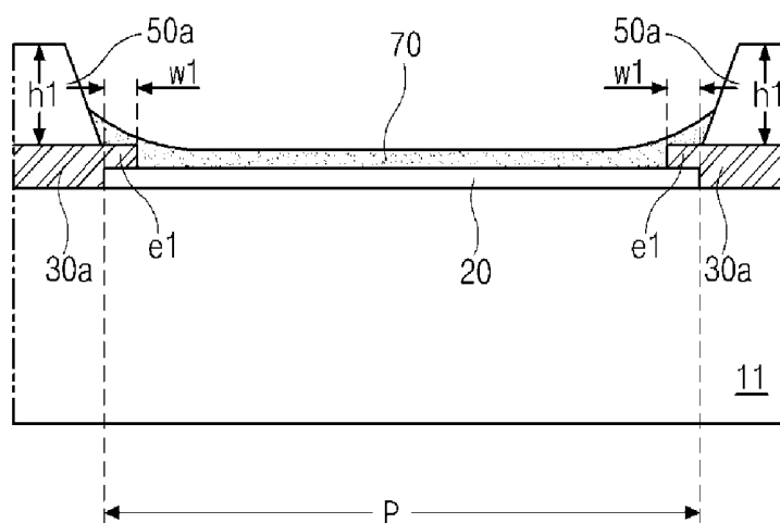
FIG. 2 RELATED ART
